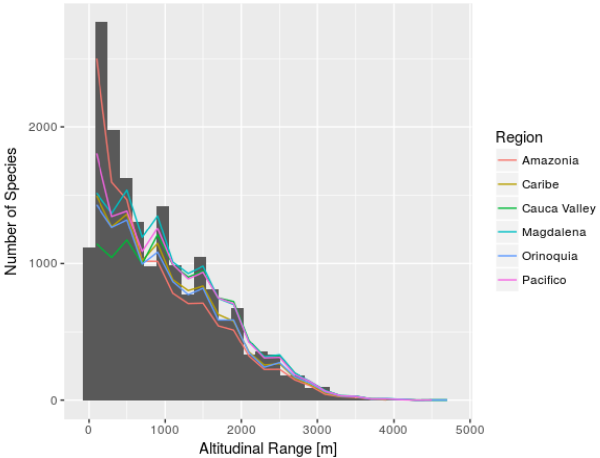
Figure A2: Altitudinal Range distribution of Colombia's vascular plants (in grey). For each one of the bioregions in different colors.
