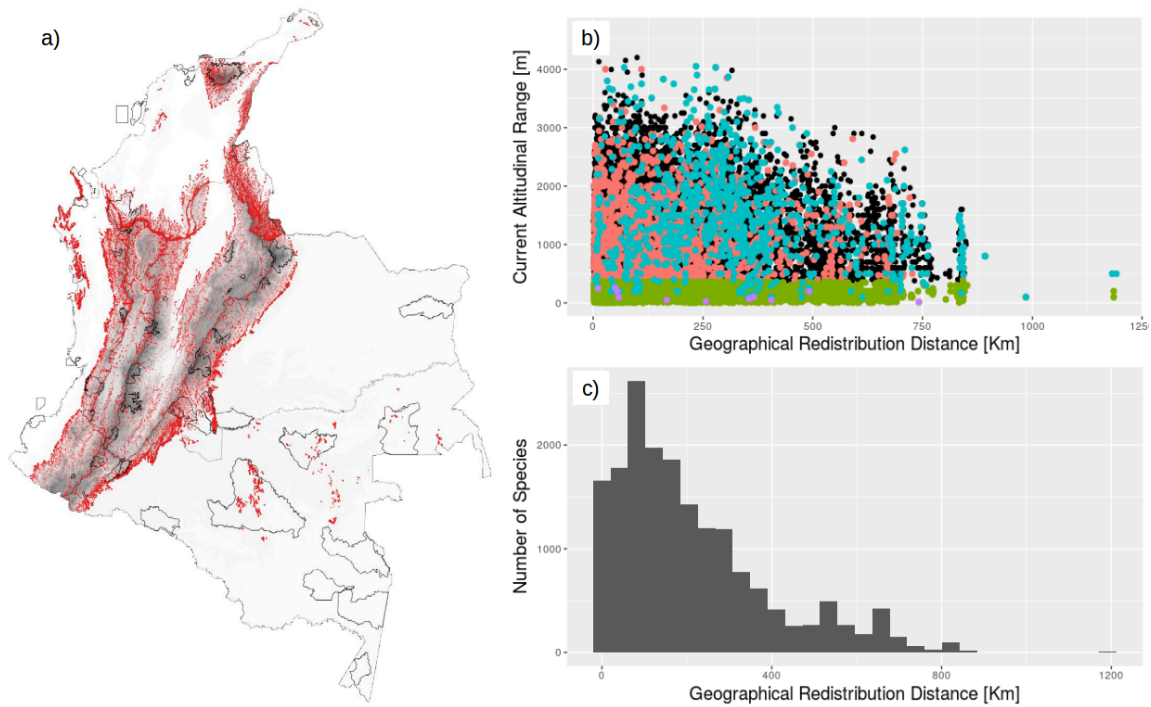
Figure 4: Geographical redistribution of the Colombia vascular Flora. a) Future migration hotspots, red points show the predicted places where species would arrive under a 2°C warming. Black polygons show the National Parks of Colombia and grey polygons denote the biogeographic regions. Grey shading shows the Colombian topography. b) Geographical redistribution distance vs. altitudinal range of Colombian vascular plant species. In orange: species affected by lowland biotic attrition. In blue: species affected by range shift gaps. In green: species affected by range contraction. In purple: species affected by mountaintop extinction. The six species on the extreme right (i.e. Diplostephium ritterbushii , Jalophila ecuadorensis , Loricaria colombiana , Myrosmodes ustulata , Myrosmodes ustulatum , Aciachne flagellifera , Lachemilla rupestris ) are particularly vulnerable because of their small altitudinal range and their enormous displacement distance for conserving their thermal niche. c) Histogram of the geographical redistribution distances of Colombian vascular plant species under 2°C warming.
