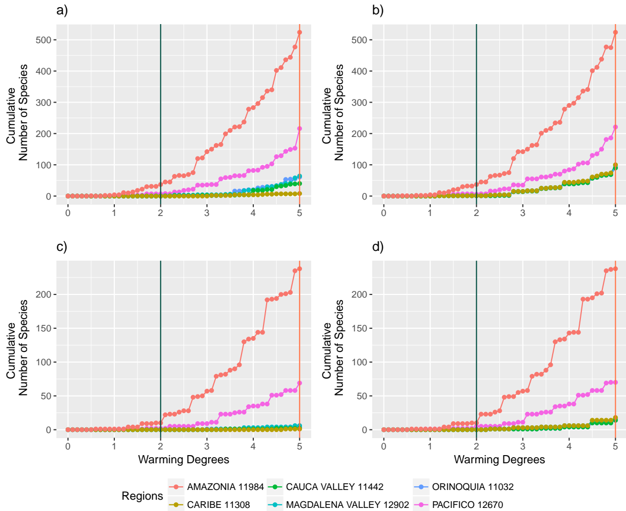
Figure 2: Cumulative number of species affected by: a) Range shift Gaps and Range Contraction under S1. b) Range Shift Gaps and Range Contraction under S2. c) Range shift gaps and mountaintop extinction under S3. d) Range shift gaps and mountaintop extinction under S4. The total number of species for each region as recorded in the Colombian Plant Catalog is provided in the legend.
