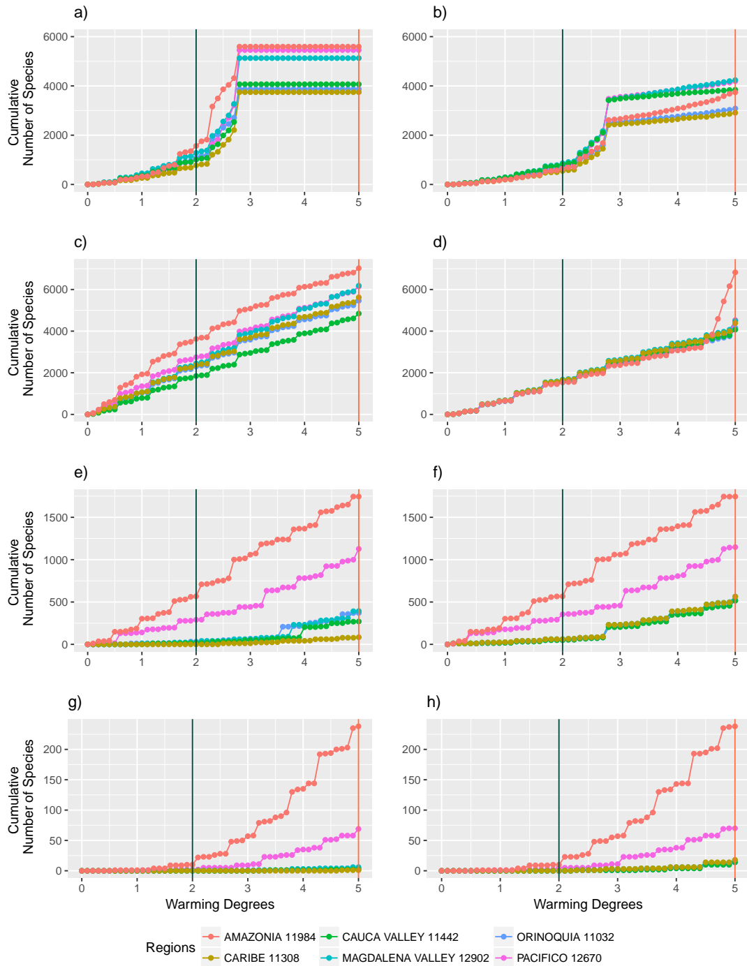
Figure 1: Cumulative number of species affected by: a) Lowland biotic attrition under the S1 scenario. b) Lowland biotic attrition under the S2 scenario. c) Range Shift Gaps under S1. d) Range Shift Gaps under S2. e) Range Contraction under S3. f) Range Contraction under S4. g) Mountaintop extinction under S3. h) Mountaintop extinction under S4. The total number of species for each region as recorded in the Colombian Plant Catalog is provided in the legend.
