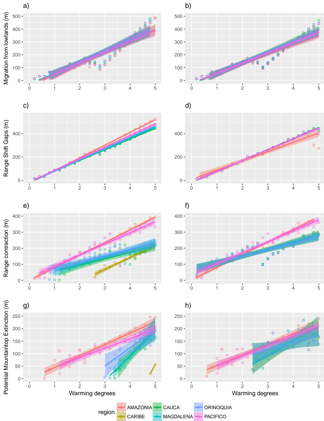
Figure 3: Average number of meters species will be affected in each bioregion: a) Lowland biotic attrition under S1. b) Lowland biotic attrition under S2. c) Range shift gaps under S1. d) Range shift gaps under S2. e) Range contraction under S3. f) Range contraction under S4. g) Mountaintop extinction under S3. h) Mountaintop extinction under S4. Confidence intervals of 95%
