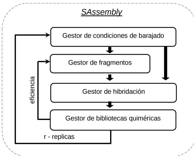
Figura 15. Arquitectura software de SAssembly.
