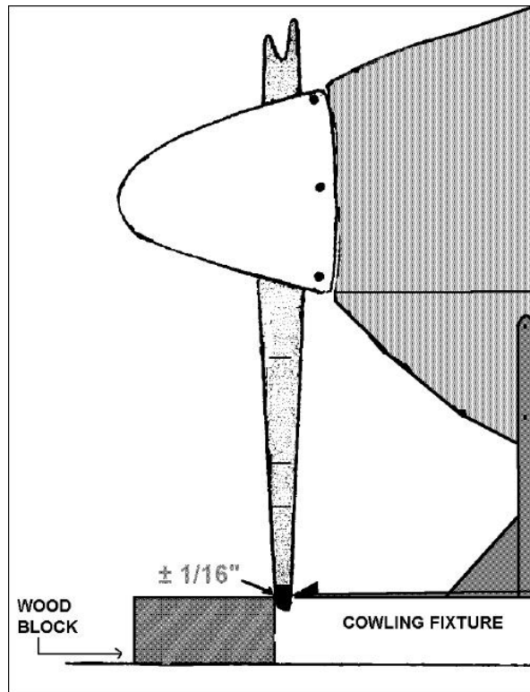
Figura 35. Propeller tracking (wood block or cowling fixture shown)
