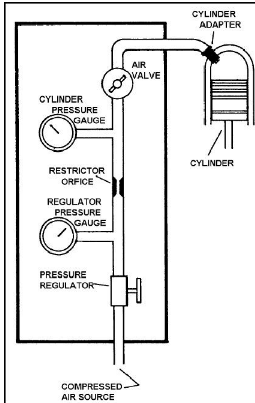
Figura 33. Schematic of differential pressure compression tester
