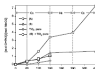
Time evolution of the [triol ketone]/[triol MoO 2 ] as a function of time in the visible light.
