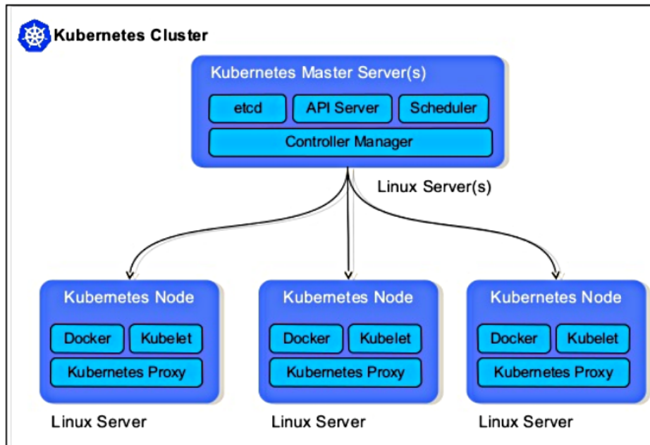
Figura 20: Kubernetes Cluster.
