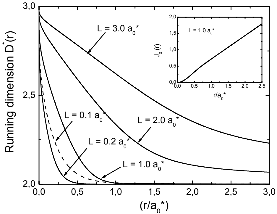
Figure 3.1 Running dimension as a function of the electron-hole separation for an exciton in a GaAs/Ga 0.7 Al 0.3 As QW and for different well width.
