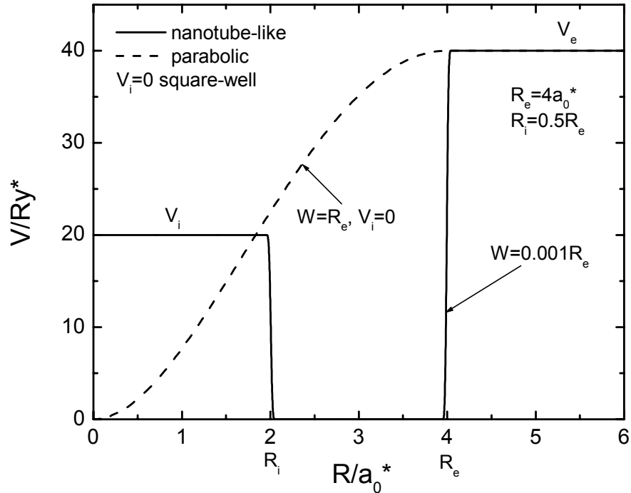
Figure 2.3 Different models of the confinement potential in a quantum wire of radius 400 Å.
