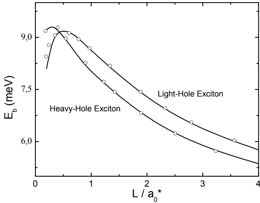
Figure 5.1 The light- and heavy-hole exciton binding energies as a function of the GaAs/Ga 0.7 Al 0.3 As QW width. Open circles correspond to calculations from Ref. 6
