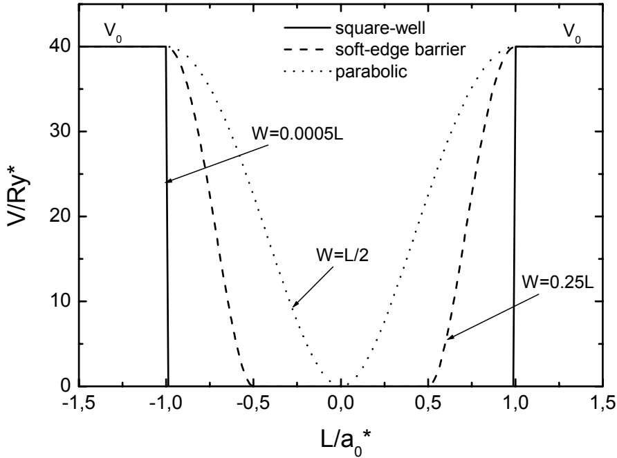
Figure 2.2 Confinement potentials for a QW of width 200 Å modeled by using equation (2.21).
