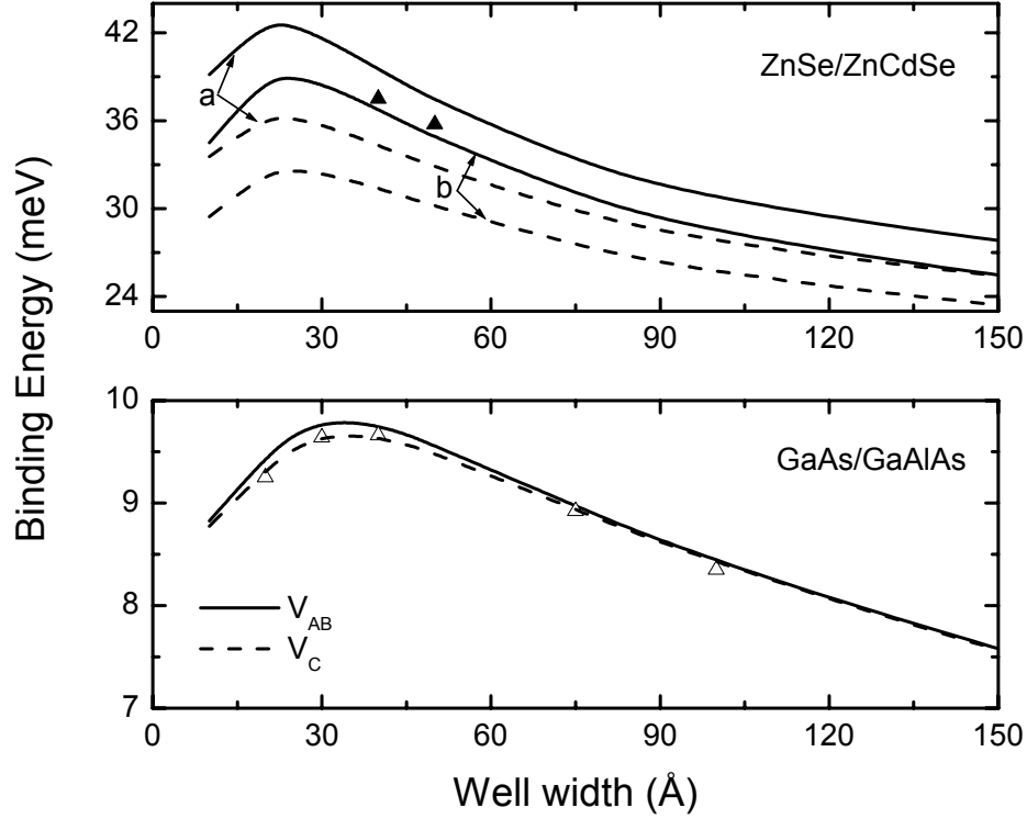
Figure 4.1 Exciton binding energies as a function of the well width for ZnSe/Zn 0.69 Cd 0.31 Se (top) and GaAs/Ga 0.7 Al 0.3 As (bottom) quantum wells. Solid curves correspond to values obtained by using the Aldrich and Bajaj V_{AB} potential for exciton-phonon interaction and dashed curves to those with Coulomb potential V_C . In the upper plot, a and b denote results as obtained with Luttinger parameters derived by Hölscher et al., and Sermage and Fishman [64–65] respectively. Open triangles correspond to theoretical calculations from Ref. [57] and solid triangles to experimental data from Ref. [61].
