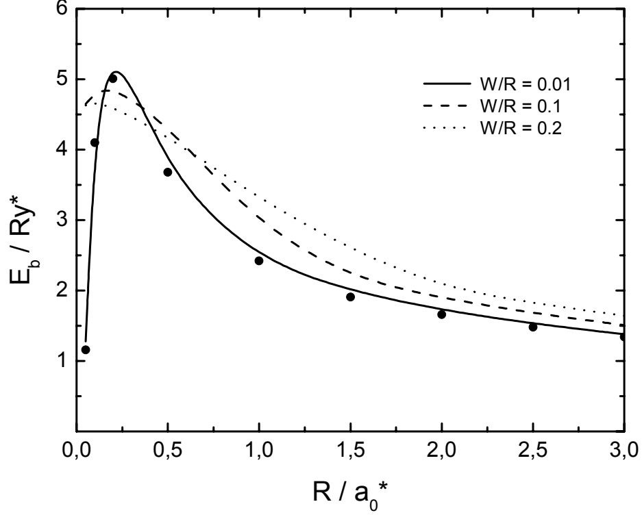
Figure 3.4 Ground state binding energy of an exciton in a GaAs/Ga 0.7 Al 0.3 As QWW as a function of the wire radius, for a model with rectangular potential (solid lines) and soft-edge barrier (dashed and dotted lines). Solid circles (•) correspond to calculations from Ref. [8].
