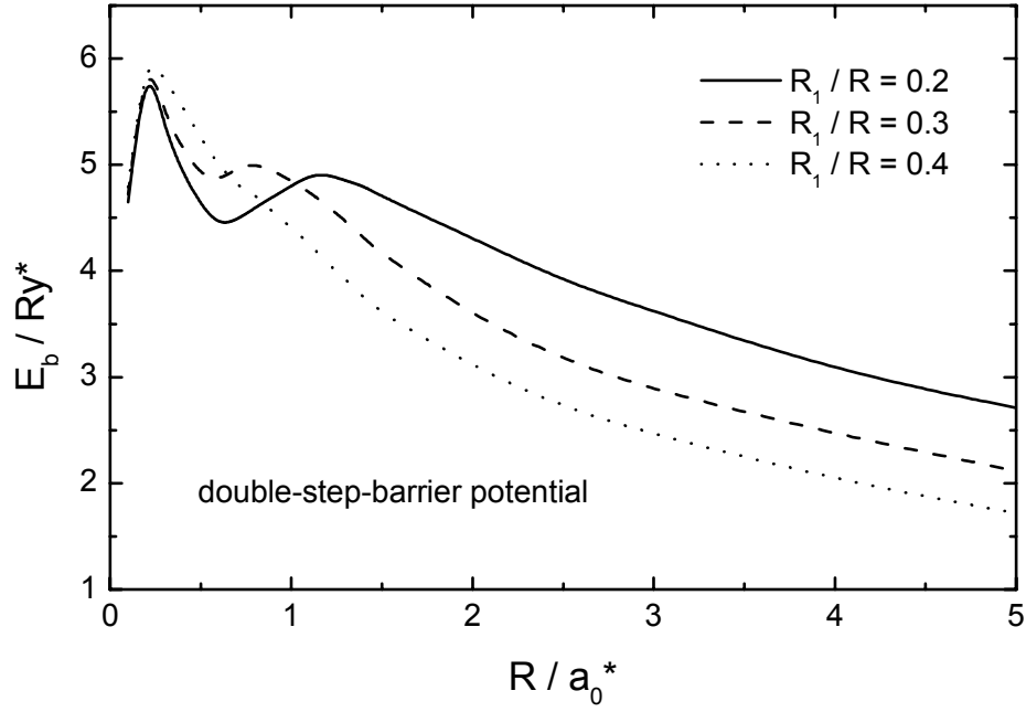
Figure 3.5 Ground state binding energy of an exciton in a GaAs/Ga 0.8 Al 0.2 As/Ga 0.55 Al 0.45 As coaxial QWW as a function of the wire radius, for a model with double-step quantum well potential.
