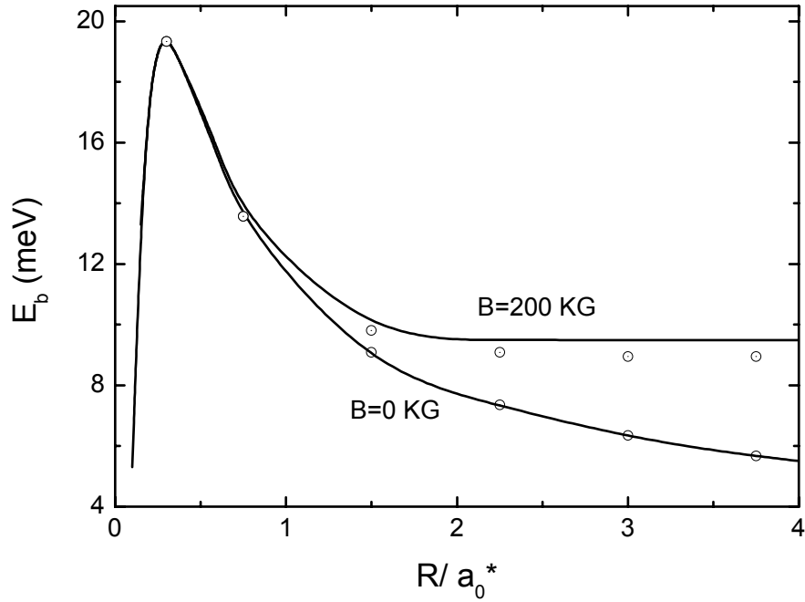
Figure 5.3 Heavy-hole exciton binding energy as a function of the wire radius with and without magnetic field. Our results (solid lines) are compared with theoretical data from Ref. 8 (open circles)
