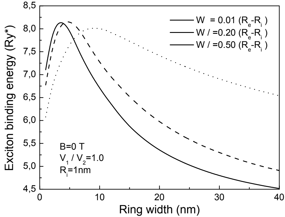
Figure 5.7 Exciton binding energy as a function of the ring width, for three different profiles of the potential barriers.
