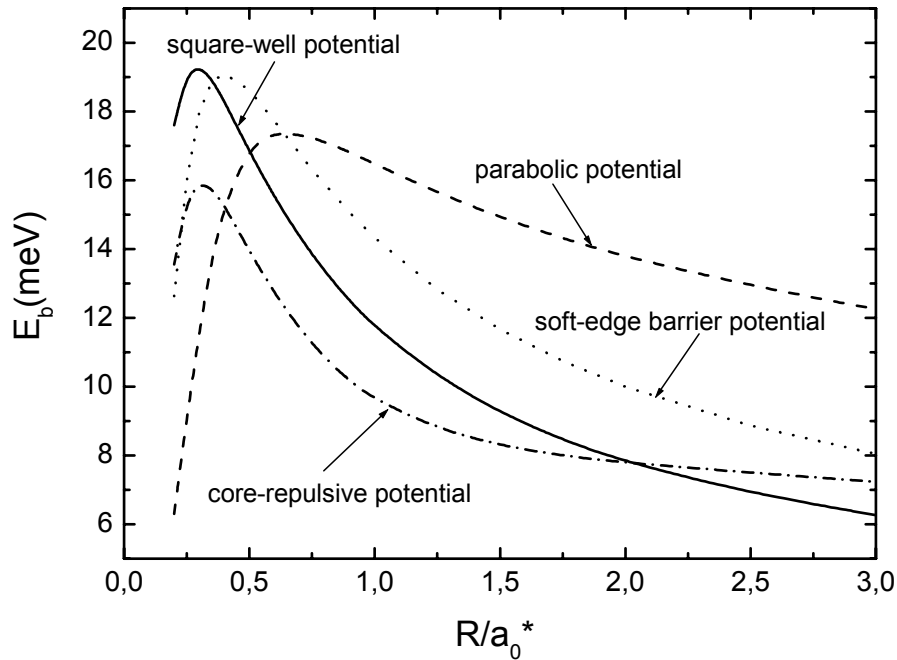
Figure 5.5 Exciton binding energies in GaAs/Ga 0.7 Al 0.3 As cylindrical QWWs with different confinement potential shapes as a function of the wire radius.
