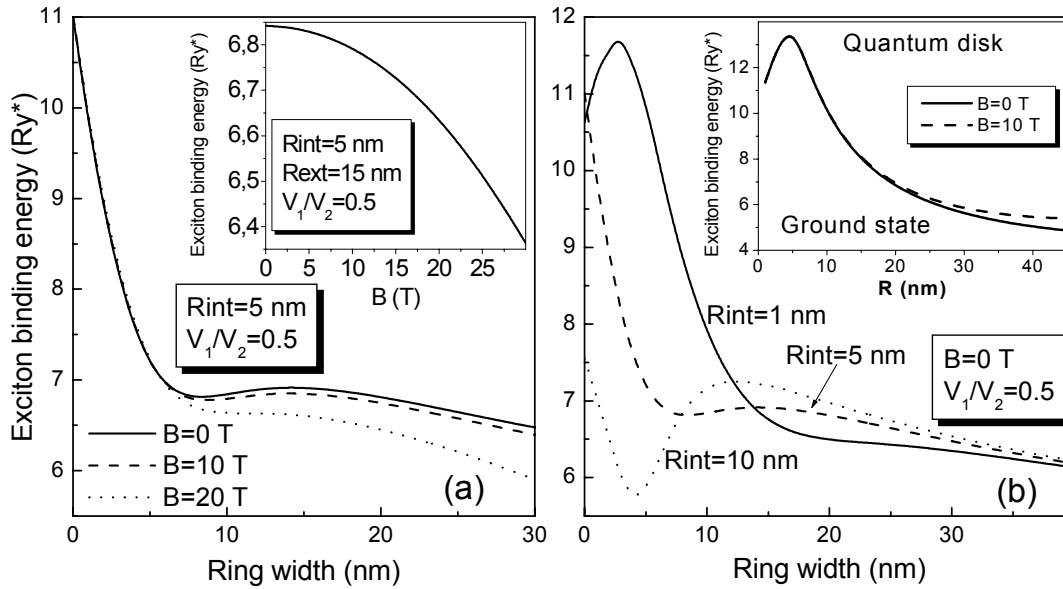
Figure 5.6 Exciton binding energy as a function of the ring width for different values of the magnetic field and core's radius. Inset in (a) shows the binding energy as a function of the magnetic field for a given ring width and in (b) shows the exciton binding energy in a quantum disk as a function of the disk radius.
