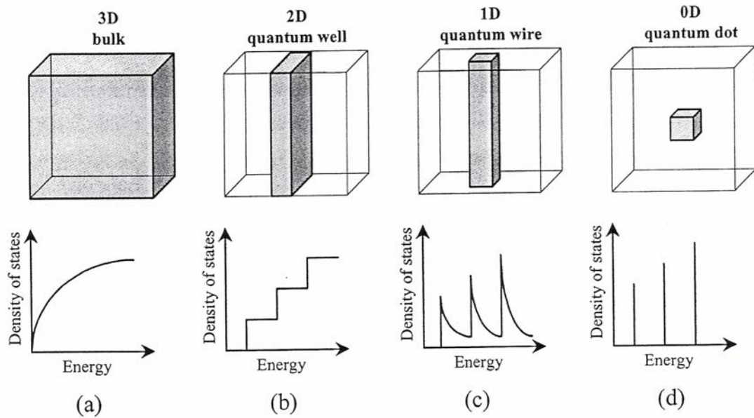
Figure 1.1 Density of states for ideal crystal structures having different dimensions: (a) three-dimensional or bulk, (b) two-dimensional or quantum well, (c) one-dimensional or quantum wire and (d) zero-dimensional or quantum dot.
