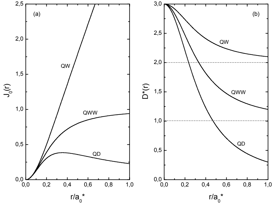
Figure 2.1 The radial part of the Jacobian (a) and running dimension (b) dependences on the electron-hole separation in QW, cylindrical QWW and spherical QD.
