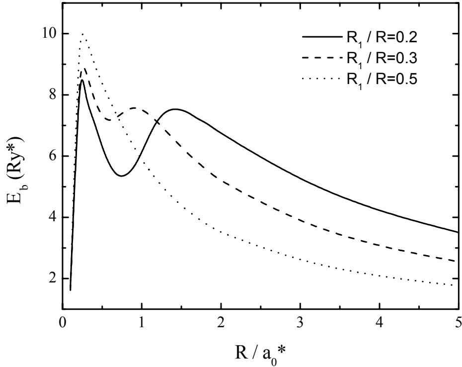
Figure 3.7 Ground state binding energy of an exciton in a GaAs/Ga 0.8 Al 0.2 As/Ga 0.55 Al 0.45 As spherical QD as a function of the wire radius, for a model with double-step quantum well potential.
