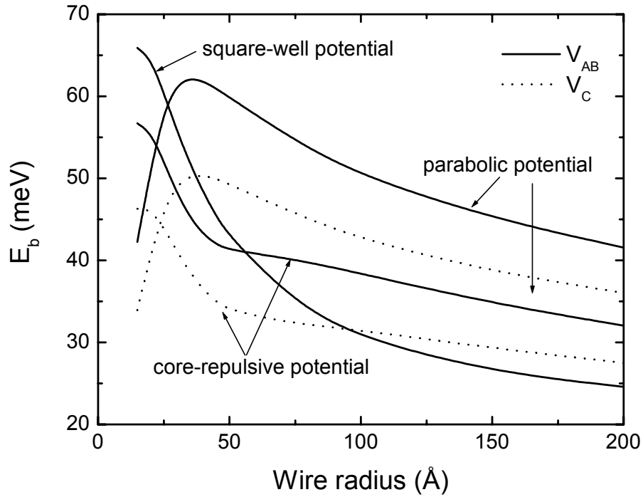
Figure 4.3 Binding energies for exciton in ZnSe/Zn 0.69 Cd 0.31 Se quantum wires as a function of the heterostructure sizes and for different confinement potential shapes. Solid curves correspond to values obtained by using the Aldrich and Bajaj V_{AB} potential for exciton-phonon interaction and dotted curves to those with Coulomb potential V_C .
