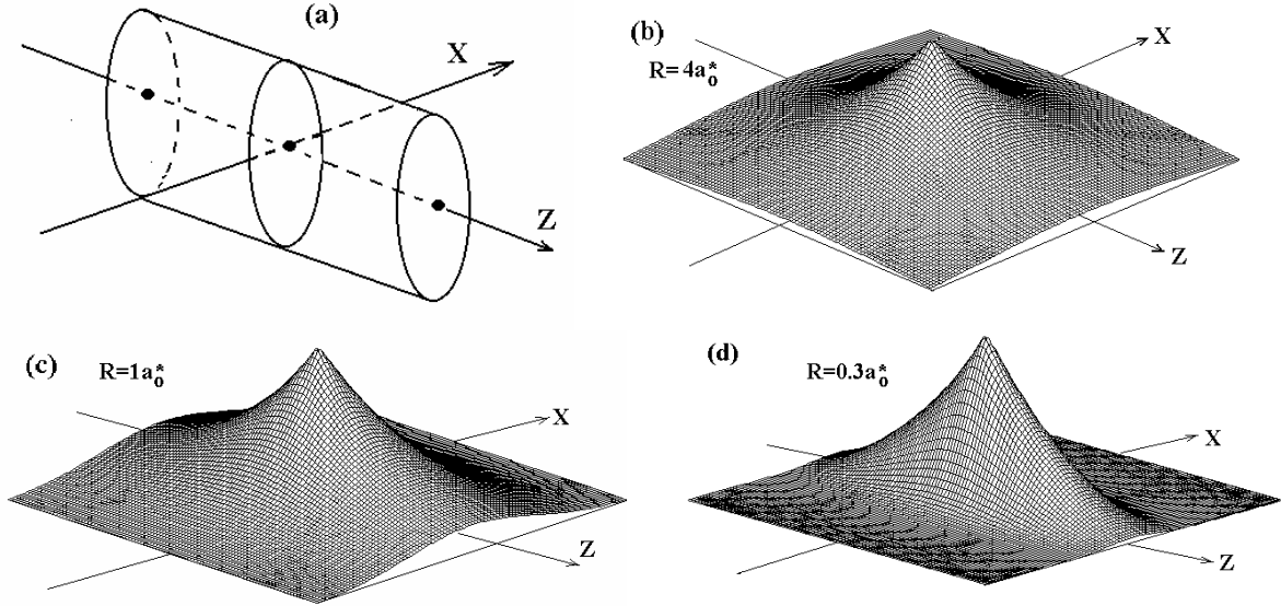
Figure 5.4 Schematic representation of the electron conditional probability density in the x - z plane, for different QWW radii: (b) R = 4.0a_0^* , (c) R = 1.0a_0^* , (d) R = 0.3a_0^* for the heavy-hole exciton with the fixed hole position at the wire axis.
