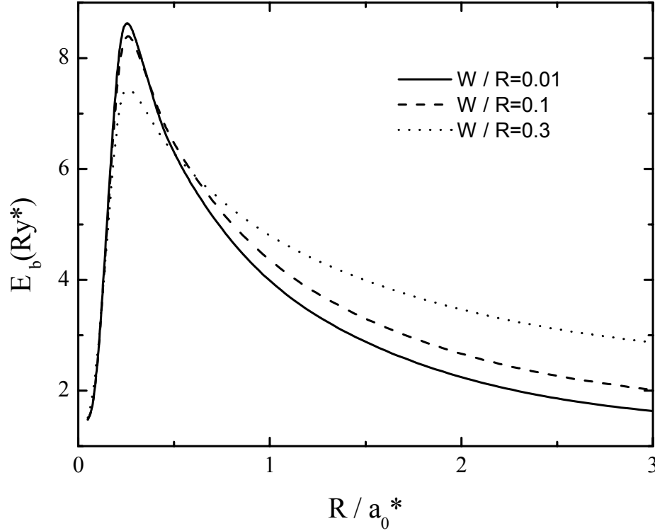
Figure 3.6 Ground state binding energy of an exciton in a GaAs/Ga 0.7 Al 0.3 As spherical QD as a function of the dot radius for different soft-edge barrier potentials.
