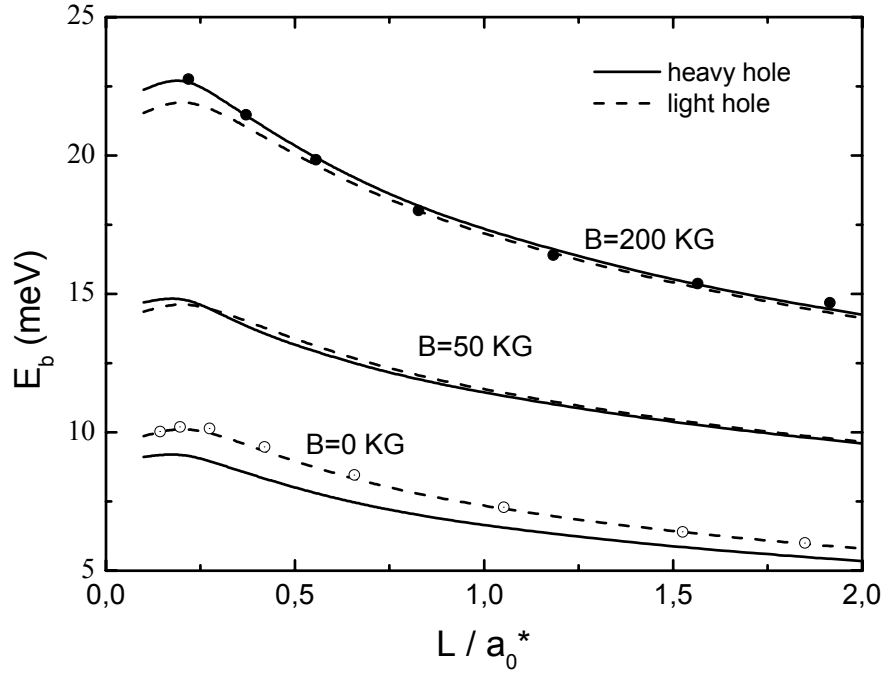
Figure 5.2 The light- and heavy-hole exciton binding energies as a function of the GaAs/Ga 0.7 Al 0.3 As QW width for different magnetic field strengths. Open circles correspond to calculations from Ref. 7
