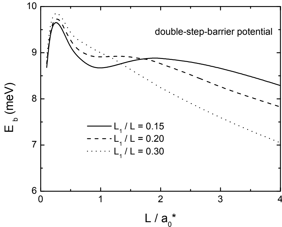
Figure 3.3 Exciton ground state binding energies as a function of the well width in a \text{GaAs}/\text{Ga}_{0.8}\text{Al}_{0.2}\text{As}/\text{Ga}_{0.55}\text{Al}_{0.45}\text{As} double-step QW and for several values of the internal well width L_1 .
