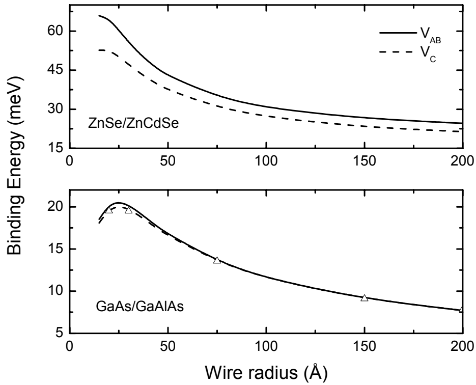
Figure 4.2 Exciton binding energies as a function of wire radius for ZnSe/Zn 0.69 Cd 0.31 Se (top) and GaAs/Ga 0.7 Al 0.3 As (bottom) quantum wells wires. Solid curves correspond to values obtained by using the Aldrich and Bajaj V_{AB} potential for exciton-phonon interaction and dashed curves to those with Coulomb potential V_C . Open triangles correspond to theoretical calculations from Ref. [8].
