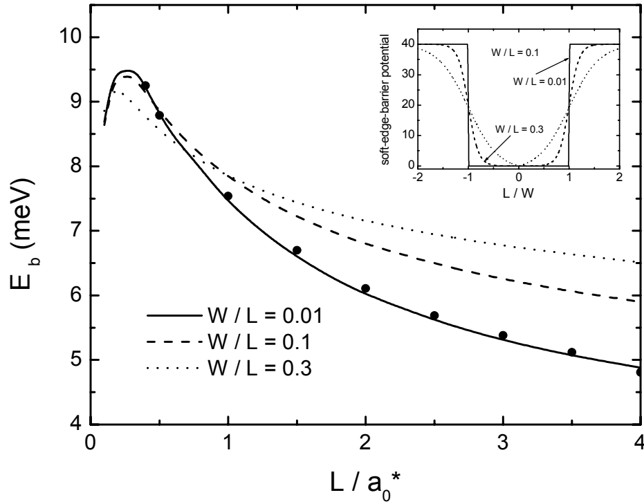
Figure 3.2 Ground state binding energy of an exciton in a GaAs/Ga 0.7 Al 0.3 As QW as a function of the well width for different soft-edge barrier potentials. Solid circles correspond to theoretical calculations from Ref. [28].
