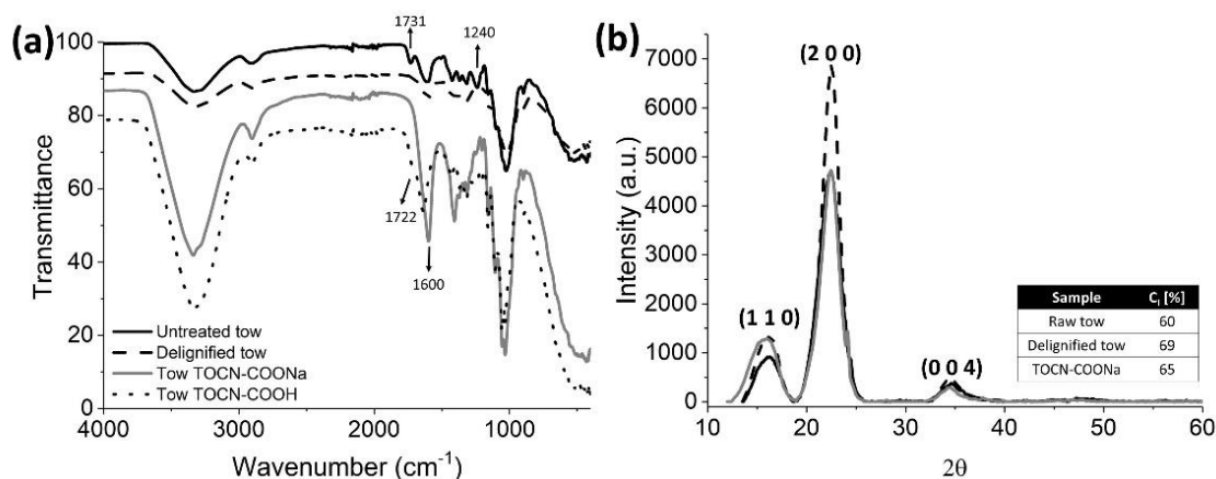
Figure 11. (a) IR-ATR spectra and (b) XRD patterns of untreated, delignified, TOCN-COO- \text{Na}^+ and TOCN-COOH Figue tow.
