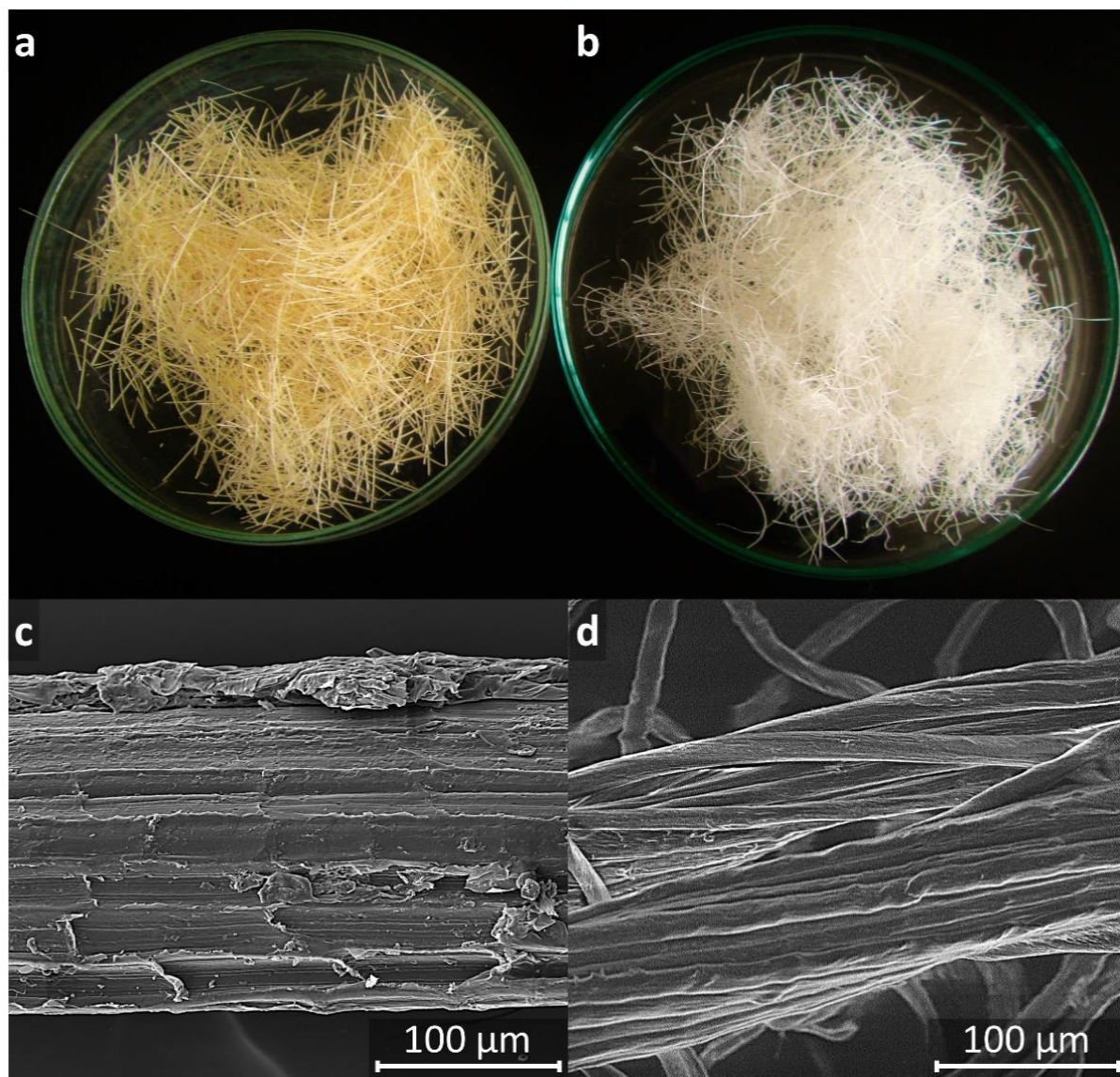
Figure 8. Images of (a) untreated and (b) delignified Figue tow. FESEM images of (c) untreated and (d) delignified Figue tow.
