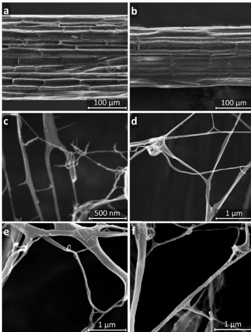
Figure 15. FESEM images of (a) untreated and (b) delignified Figue tow, (c) TOCN, (d) TOCN-P, (e) TOCN-ODA and (f) TOCN-P-ODA.
