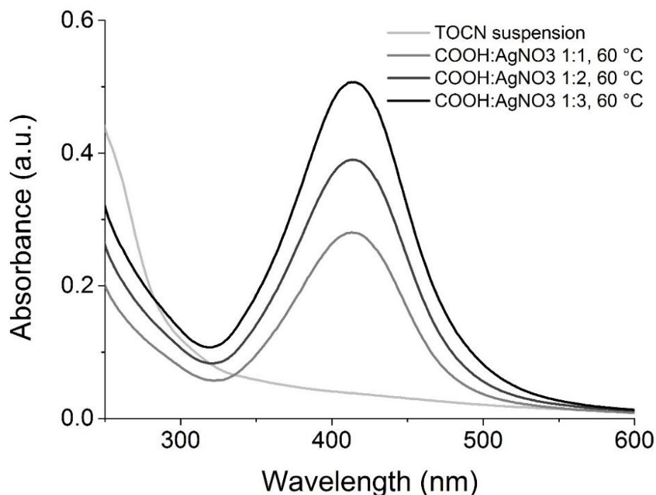
Figure 24. UV-Vis spectra of TOCN suspensions and TOCN-Ag NPs hydrogels prepared at 60 °C.
