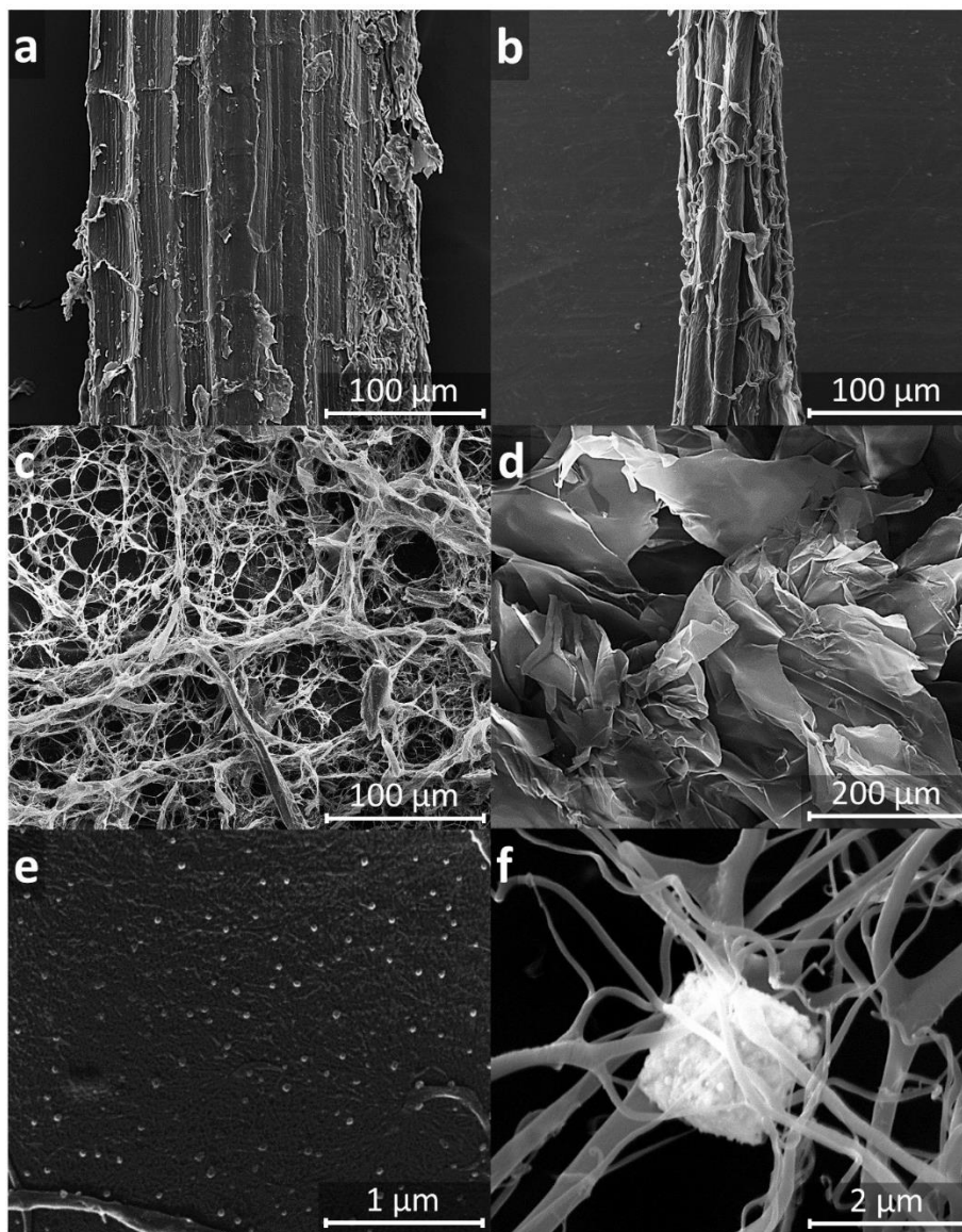
Figure 25. FESEM images of (a) raw and (b) delignified Figue tow, (c) air-dried TOCN suspension, (d) TOCN aerogels and (e) and (f) TOCN-Ag NPs aerogels.
