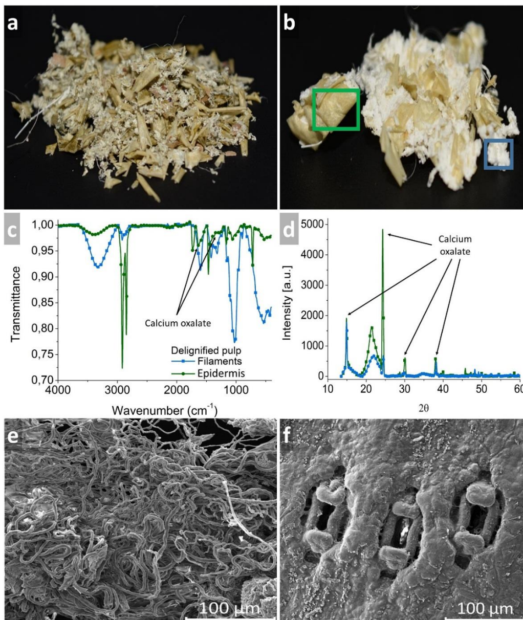
Figure 5. Optical images of (a) raw and (b) delignified Figue pulp. (c) IR spectra and (d) XRD patterns of cellulosic filaments (blue trace) and leaf epidermis (green trace) in delignified Figue pulp. FESEM images of (e) cellulosic filaments and (f) leaf epidermis in delignified Figue pulp.
