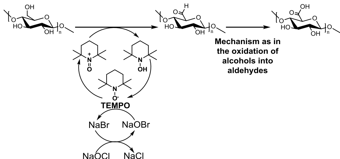
Figure 14. TEMPO-mediated oxidation of primary hydroxyls to carboxyl groups.
