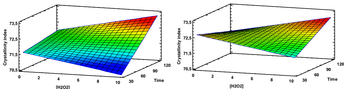
Figure 7. Crystallinity index as a function of H 2 O 2 concentration and reaction time using (a) 1% w/v and (b) 8% w/v loadings.
