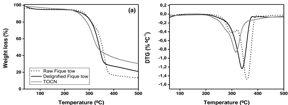
Figure 12. (a) TGA curves and (b) DTG curves for raw Fique tow, delignified Fique tow and TOCN.
