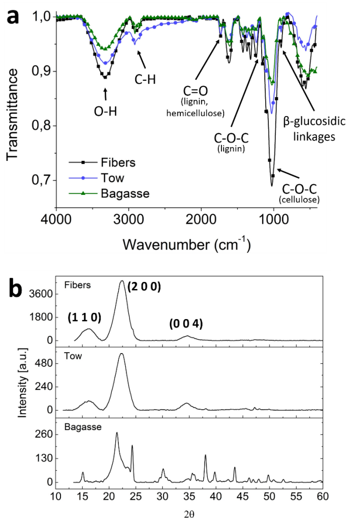
Figure 2. (a) IR spectra and (b) XRD patterns of Fique fibers, tow and pulp.
