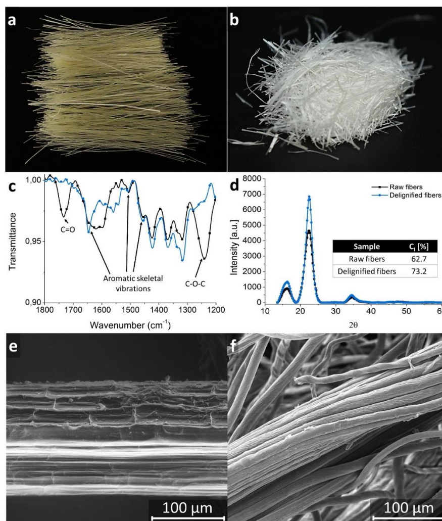
Figure 4. Optical images of (a) raw and (b) delignified Fique fibers/tow. (c) IR spectra, (d) XRD patterns and FESEM images of (e) raw and (f) delignified Fique fibers/tow.
