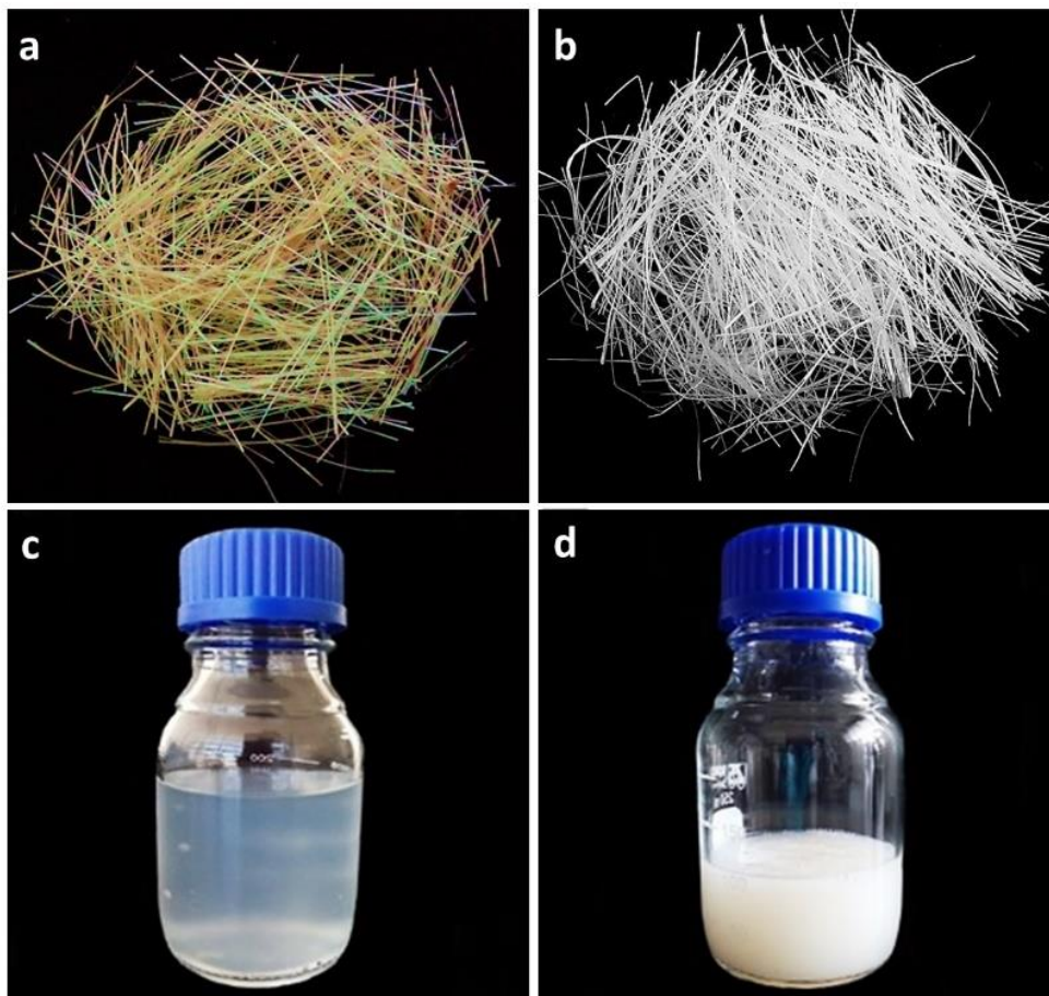
Figure 13. Images of (a) untreated and (b) delignified Fique tow, (c) TOCN in water and (d) TOCN-ODA in toluene.
