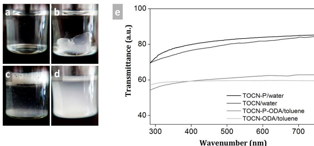
Figure 19. Images of (a) TOCN/water (b) TOCN/toluene (c) TOCN-ODA/water (d) TOCN-ODA/toluene and e) Light transmittance spectra of TOCN-(P) in water and TOCN-(P)-ODA in toluene dispersions.
