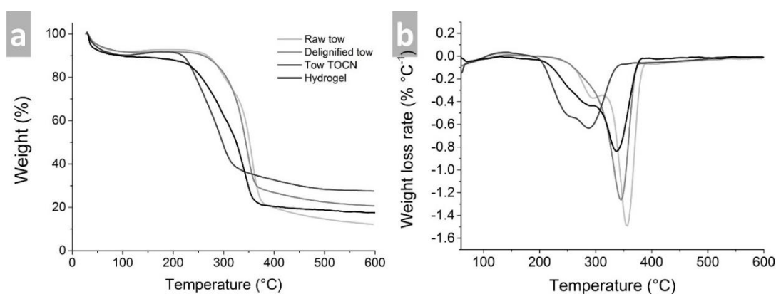
Figure 27. (a) TGA curves and (b) DTG curves for raw Fique tow, delignified Fique tow, TOCN and TOCN-Ag NPs hydrogels.
