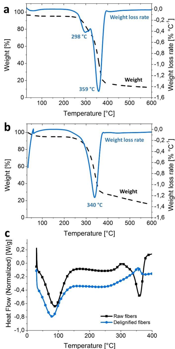
Figure 6. TGA and DTG thermograms of (a) raw and (b) delignified fibers/tow and DSC thermograms (c) for raw and delignified fibers/tow.
