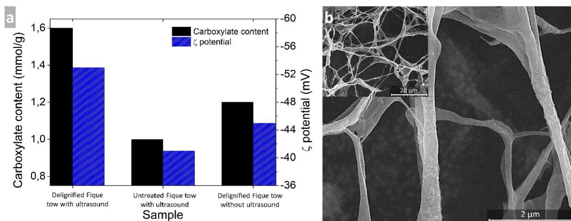
Figure 10. Fique tow TOCN: (a) \zeta potential and carboxylate contents, (b) FESEM image.
