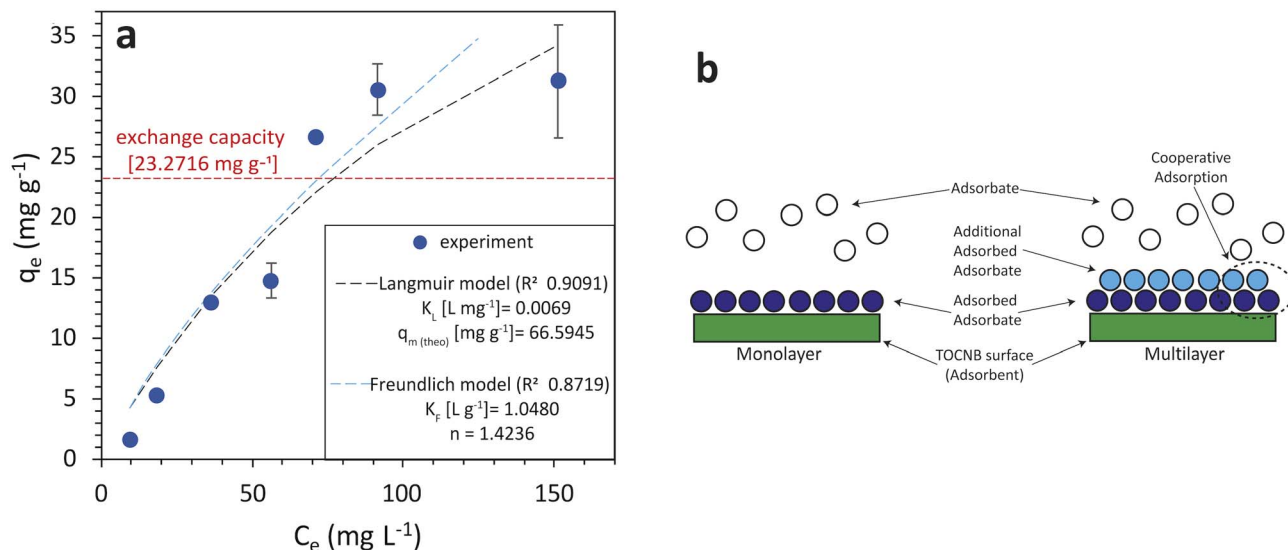
Fig. 7 (a) Experimental \text{NH}_4^+ adsorption isotherm onto TOCNB (100 mg per L \text{NH}_4^+ ; 150 rpm; pH 7; 0.25 g per L TOCNB). The data are fitted to Langmuir and Freundlich models. (b) Schematics of possible \text{NH}_4^+ /TOCNB interactions via mono and multilayer formation. Own elaboration based on Nandiyanto et al. 93
