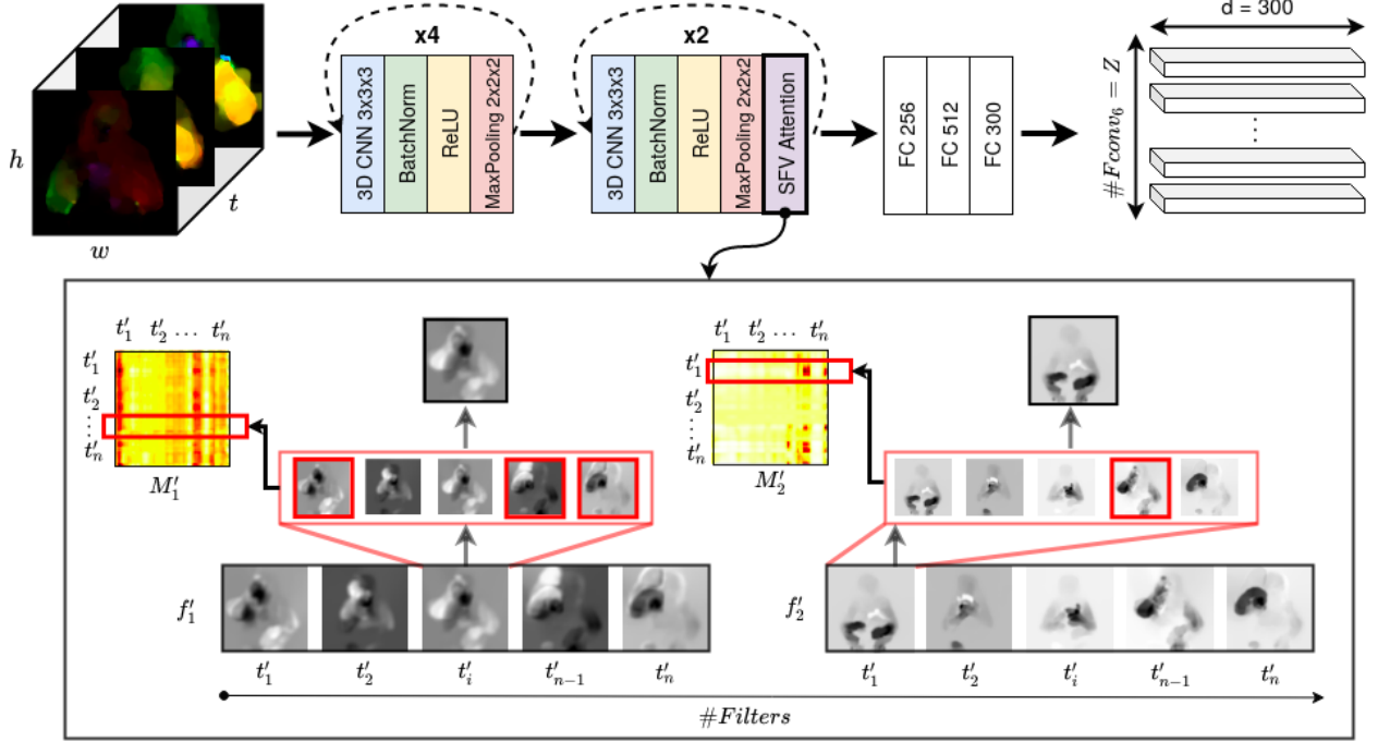
Figure 2. Structured SL Features Volumes extractor: This proposed module extracts low-level spatio-temporal features volumes through successive 3D-CNN. The SFV attention module takes each resulting convolution and applies self-attention on the whole volume by calculating an attention matrix for each filter in an independent and parallel way. Each feature frame is then related in different proportions to the other frames according to the temporal relationship between them.
