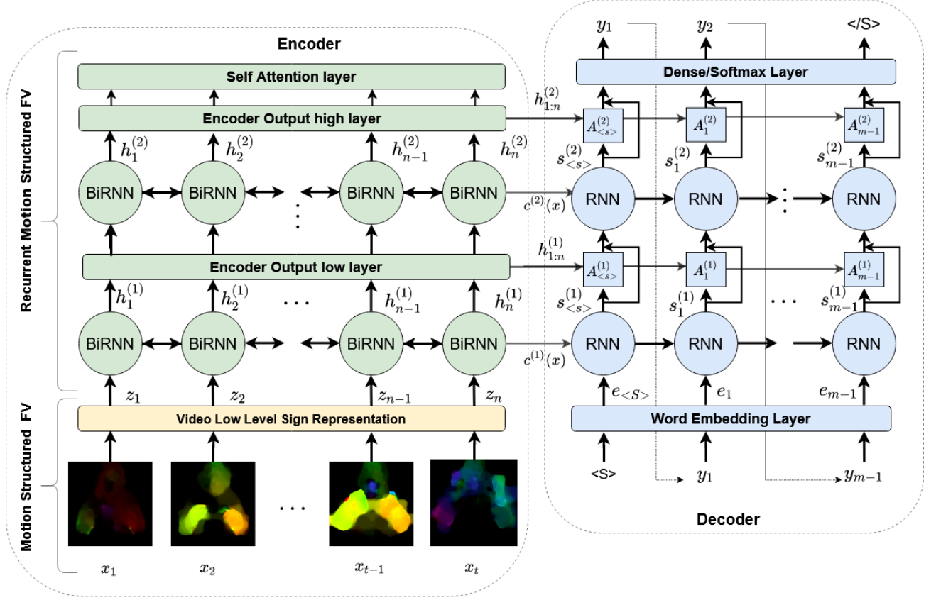
Figure 1. Proposed structured SLT architecture: Optical flow video is the input to the network. The encoder processes at low level extracting structured kinematic descriptors. Then, at a higher level, the Encoder sequentially processes the descriptors. Finally, the descriptors are passed to the Decoder to generate the translation.
