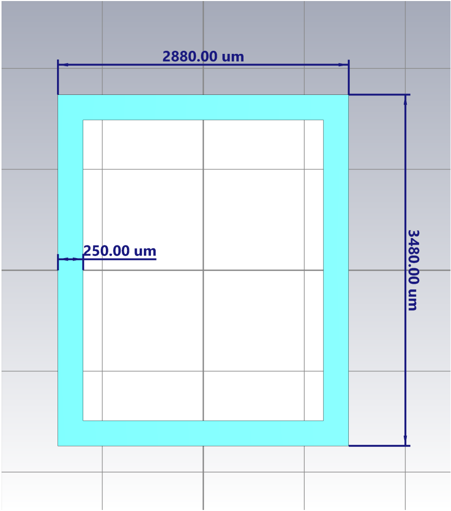
Figure 10 Antenna design in CST Studio Suite.
