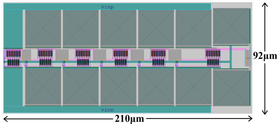
Figure 27 Full-wave rectifier layout using Magic.
