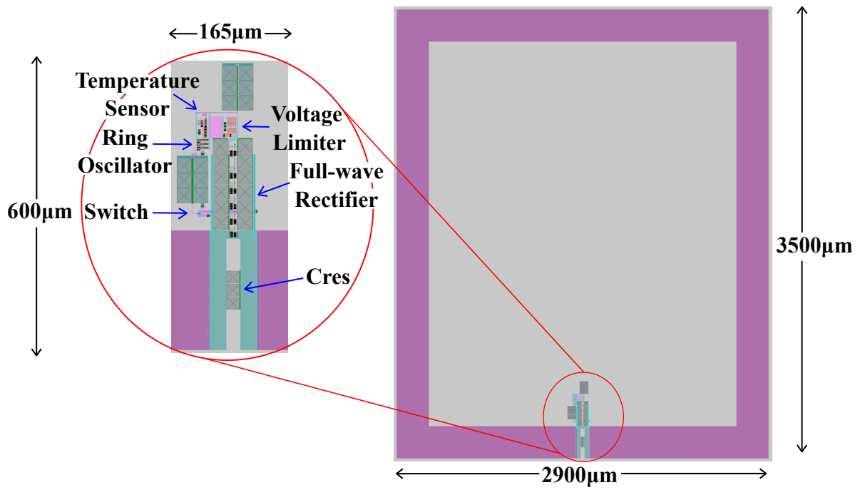
Figure 41 RFID Tag Layout performed in Magic.
