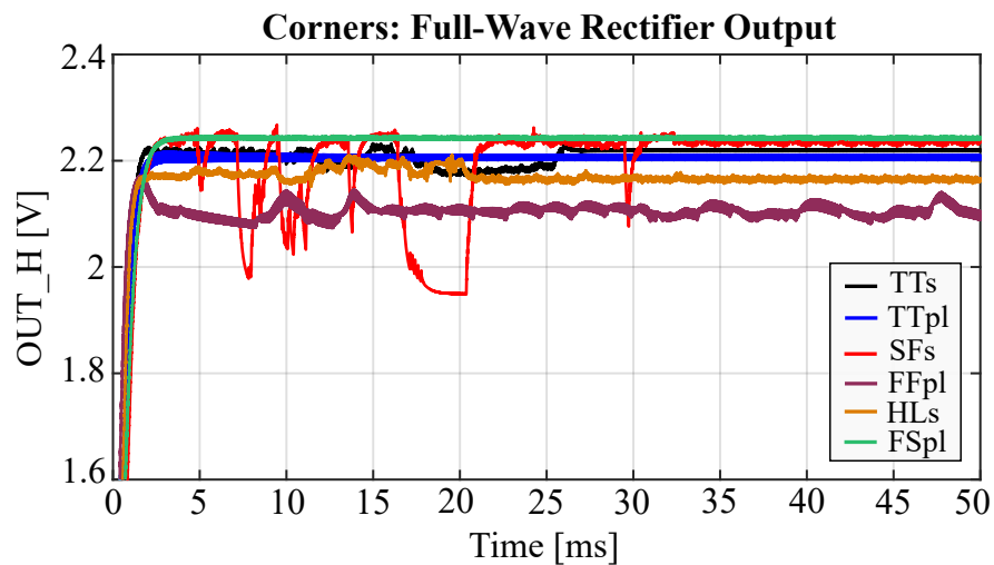
Figure 28 Corner simulation results for both schematic and post-layout netlists.
