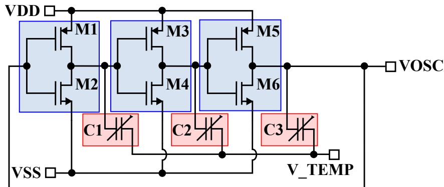
Figure 17 Ring Oscillator Schematic using varactors.
