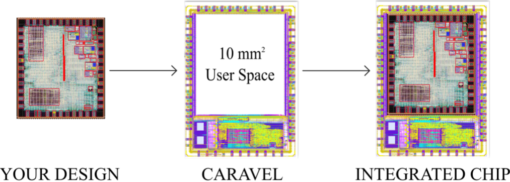
Figure 6 Connection between the user project and the Caravel.
