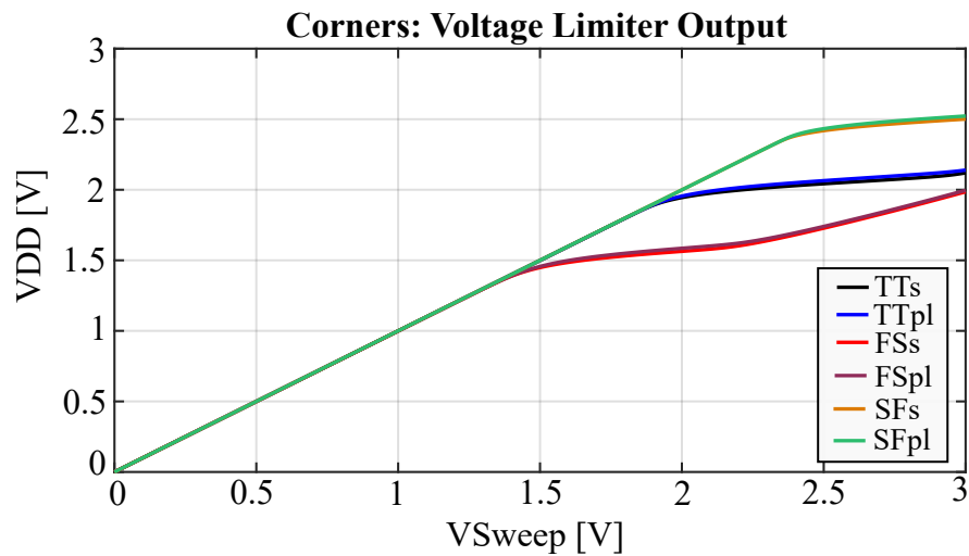
Figure 30 Corner simulation results of the Voltage Limiter for both schematic and post-layout netlists.
