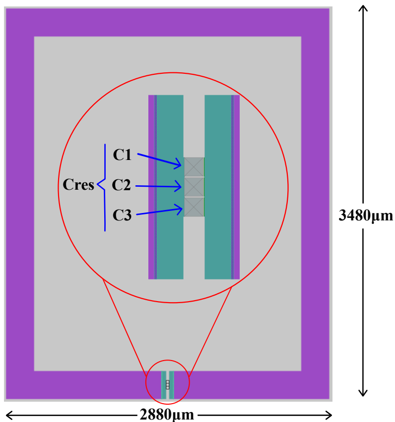
Figure 26 Layout of the Resonator using Magic.
